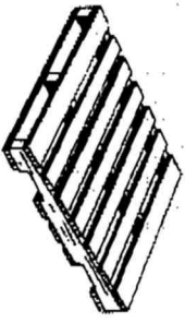
Heavy Duty Stringer Pallet Notched for Four-Way Entry
